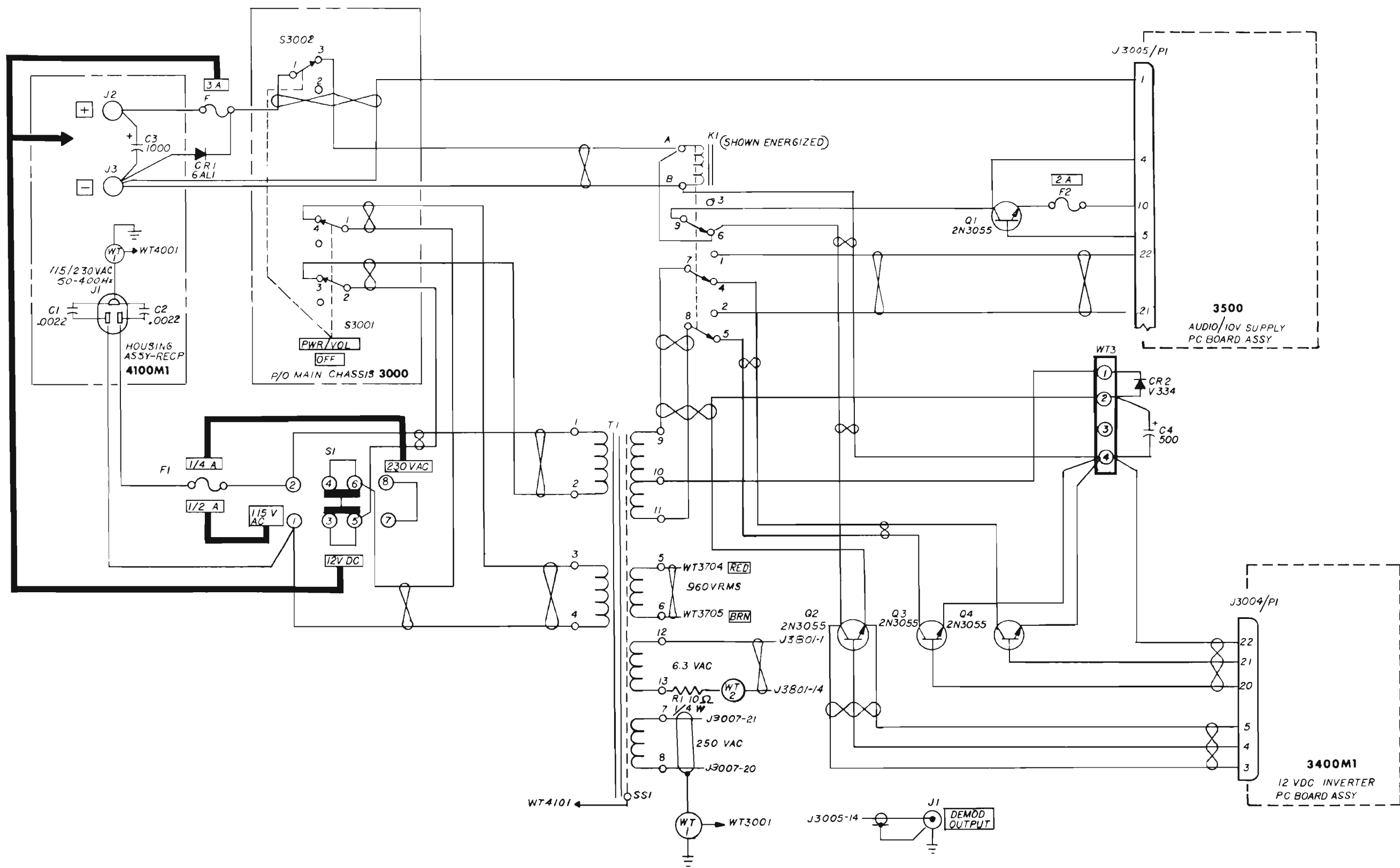
Figure 5-19. Rear Panel Interconnection Diagram, 4000 M1
